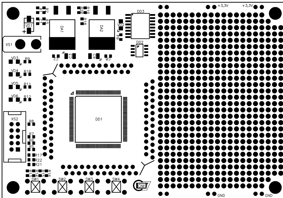
Fig. 4. External view of the printing board.
