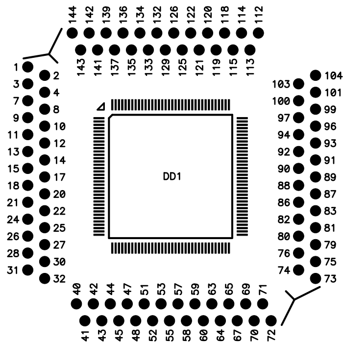
Fig. 5. Designation of mounting pads.
