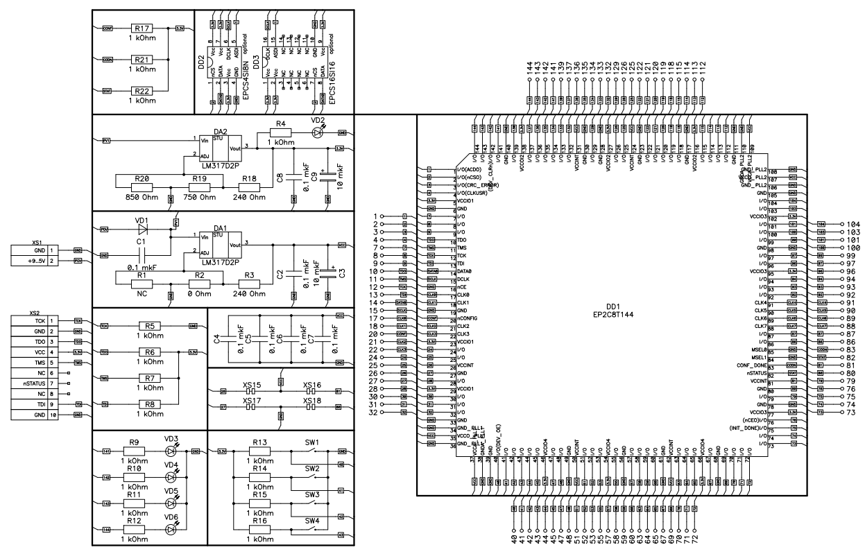
Fig. 3. The electrical scheme of LDM-EP2C8-T144
