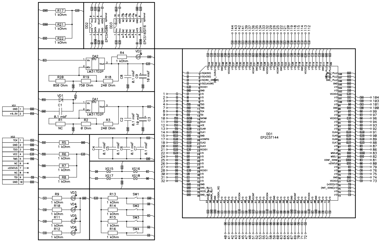
Fig. 2. The electrical scheme of LDM-EP2C5-T144
