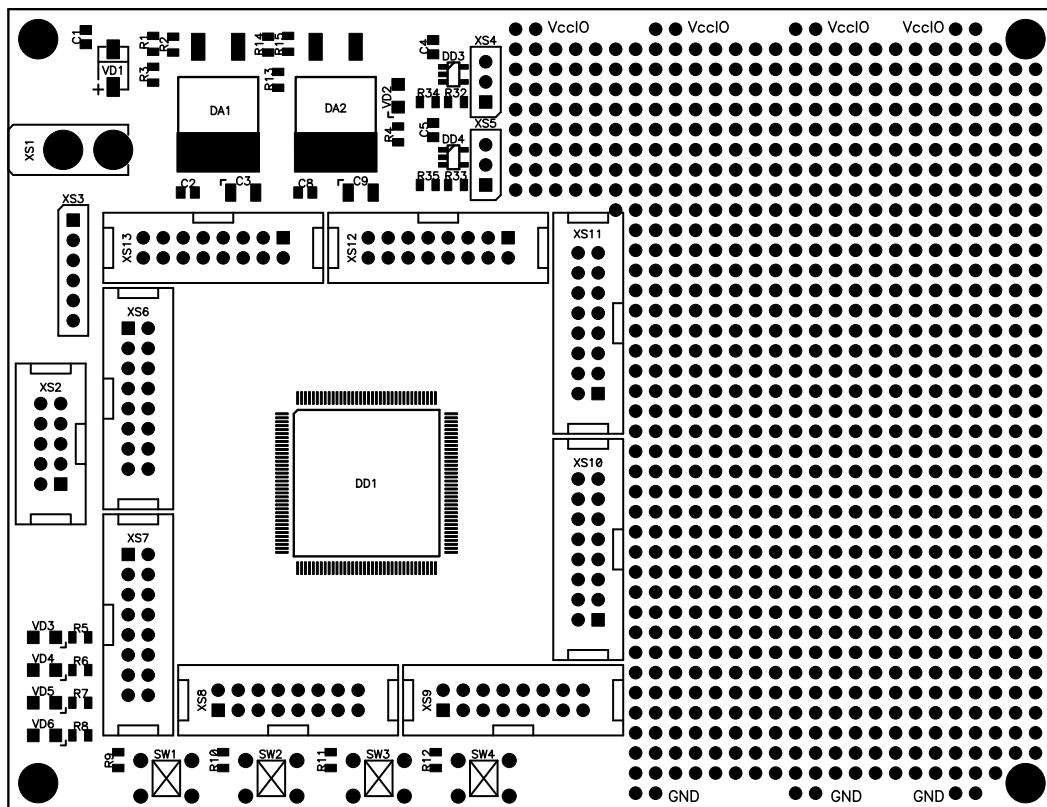
Fig. 4. External view of the printing board.
