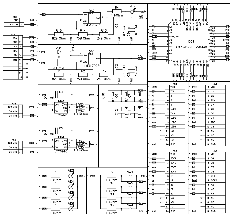
Fig. 2. The electrical scheme XB-XCR3032XL-VQ44
