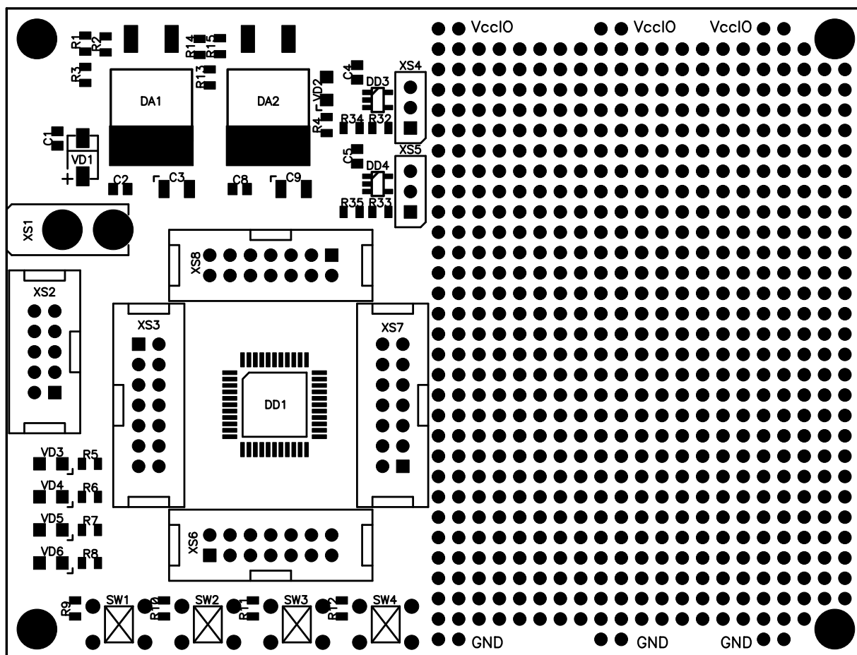
Fig. 4. External view of the printing board.
