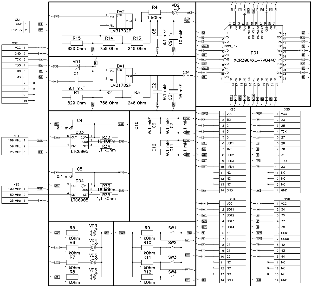
Fig. 3. The electrical scheme XB-XCR3064XL-VQ44
